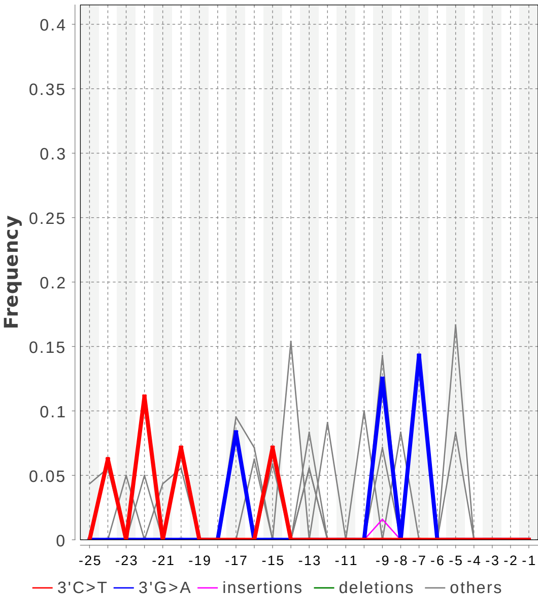
3' end
