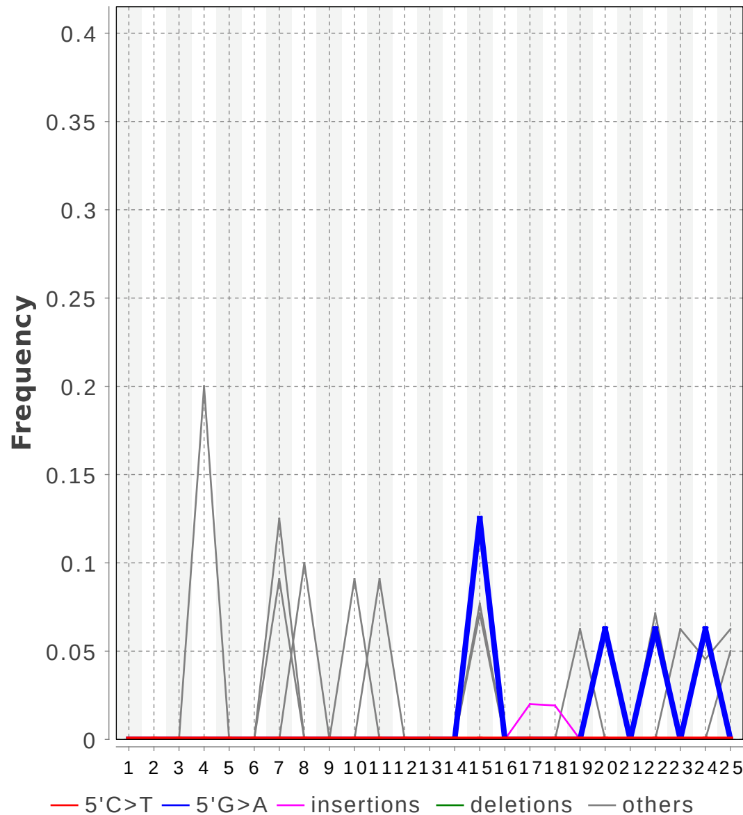
5' end
