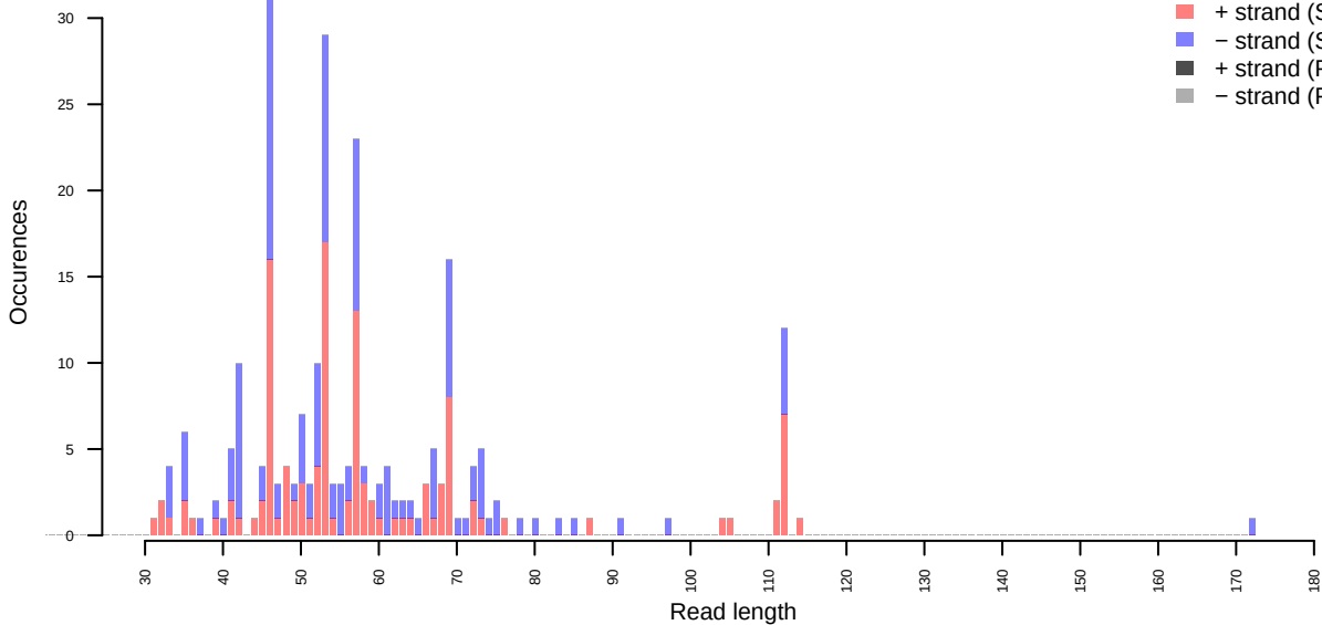
Length distribution
